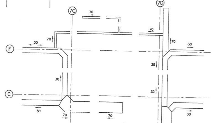
GRATING PLAN (THICKNESS IN MM. SHOWN) EDGE PROFILES, REF. DWG. W2HT/BN286
